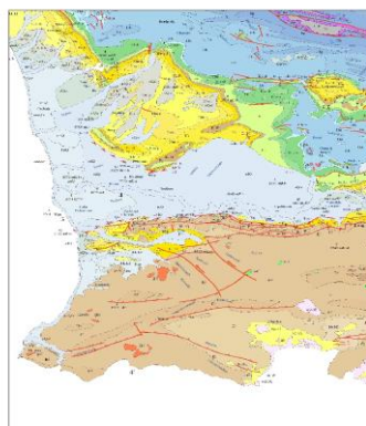
Fig. 2 Geological map
